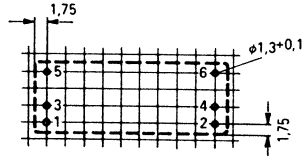
Mounting hole layout View from the wiring side
