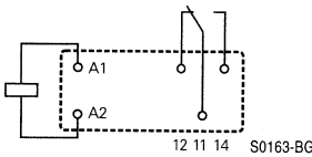
8 A and 12 A version
