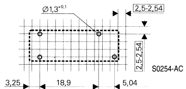
Mounting hole layout View from the wiring side
