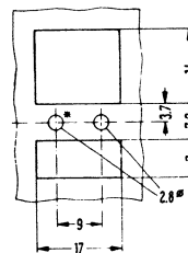
Mounting hole layout Size II
