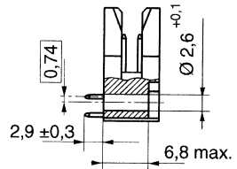
Angled tails (horizontal version)
