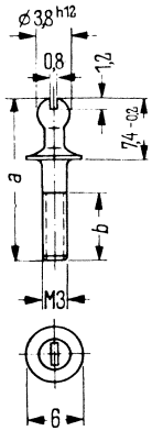
Pin
