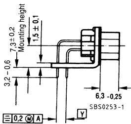
Female connector
