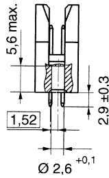
Straight tails (vertical version)
