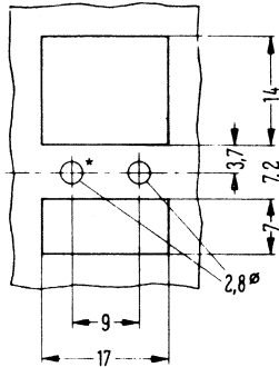
Mounting hole layout
