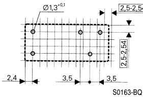
8 A and 12 A version
