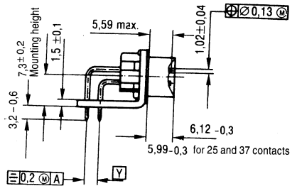
Pin connector
